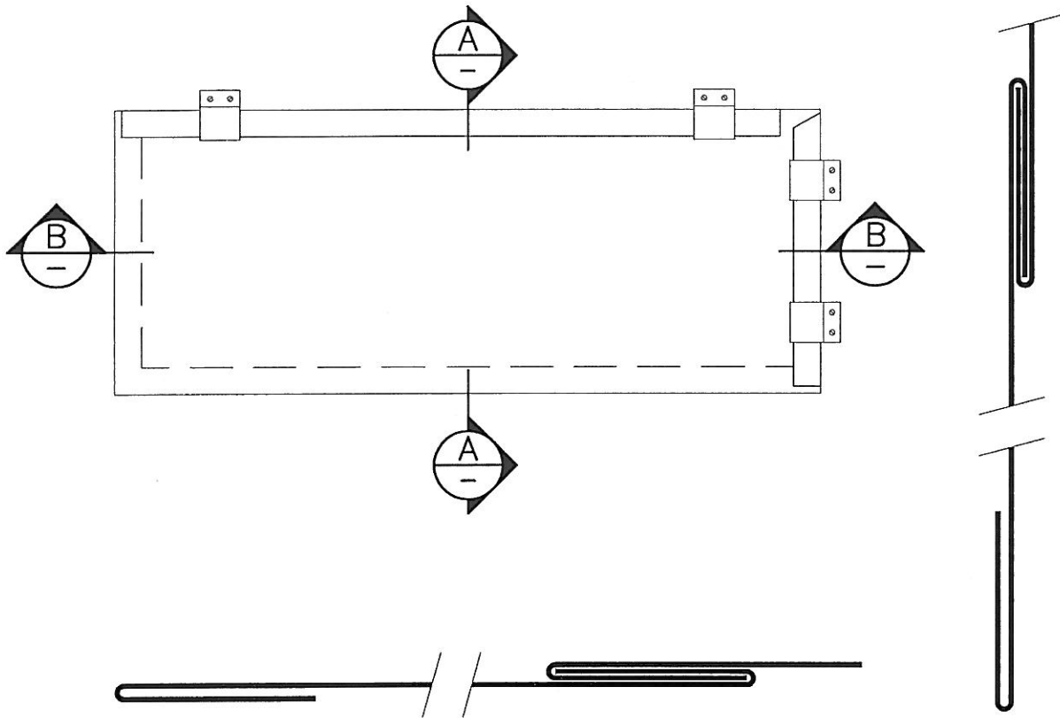
Section B-B
