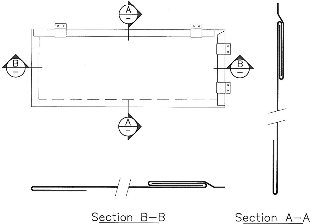
Detail 6
